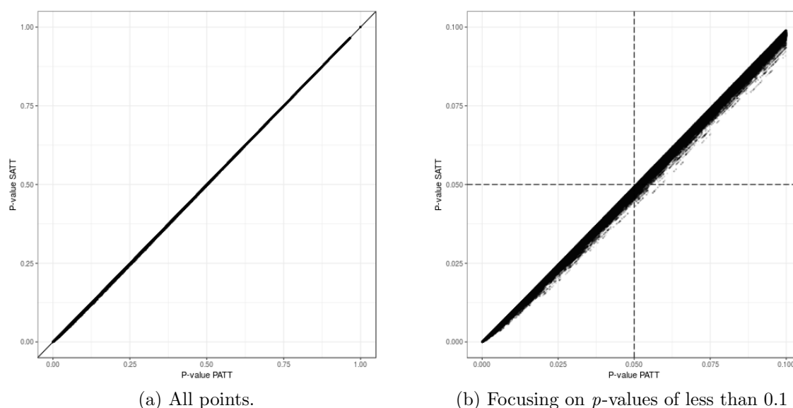
Figure 3.4: Scatter plot of p -values computed for att under infinite sampling versus p -values for att under finite sampling. Ten percent of the the over 400 million points of the grid have been randomly selected for this plot.
